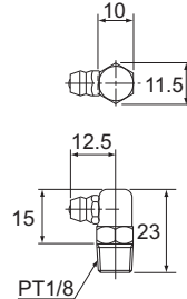
C-PT1/8
