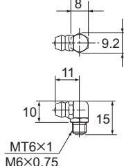
C-M6F (M6×0.75)
