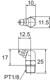
B-PT1/8
