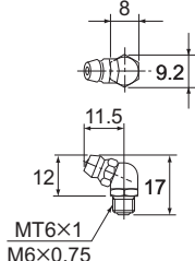
B-M6F (M6×0.75)
