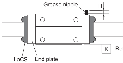
Grease nipple mounting location for models SHS, SSR, SVR/SVS, NR-X/NRS-X, SRG, and HRX
