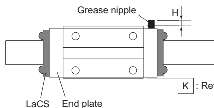
Grease nipple mounting location for models SHS, SSR, SVR/SVS, NR-X/NRS-X, SRG, and HRX
