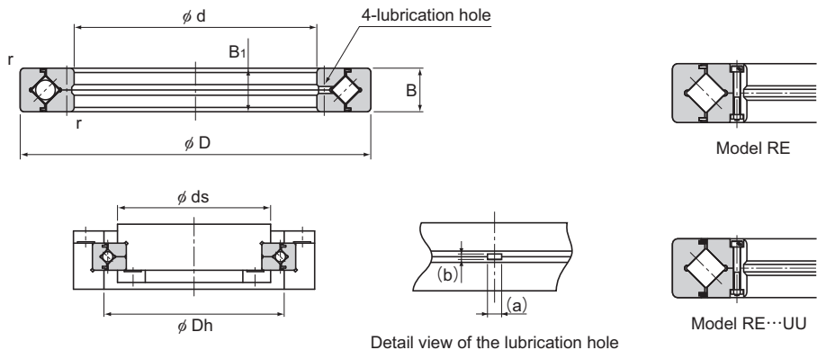
Detail view of the lubrication hole
