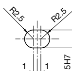
Elongated hole (detail)
