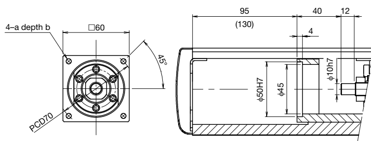
Motor bracket (detail) (symbol: A, B)
