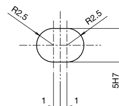
Elongated hole (detail)
