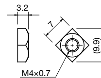
Square Nut (x8)
