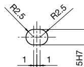
Elongated hole (detail)
