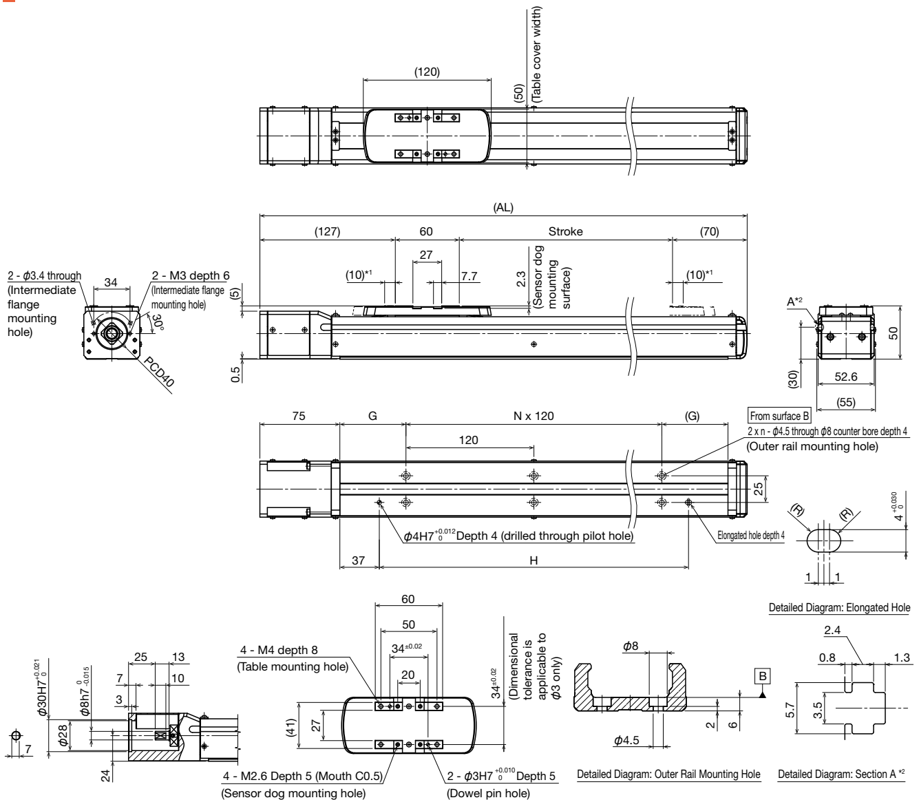
Detailed drawing of motor mounting part (when A0 is selected) *3
