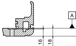
Counter-bore hole on base (detail)
