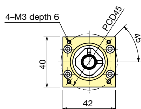
Arrow F view
